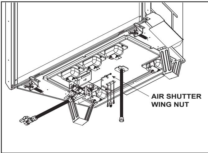
Figure 9.1 Air Shutter
