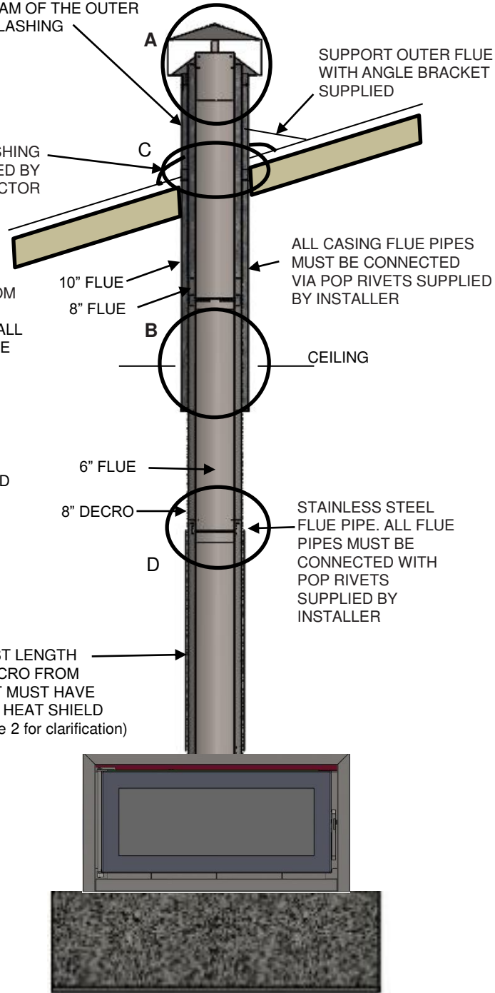
FRONT VIEW
