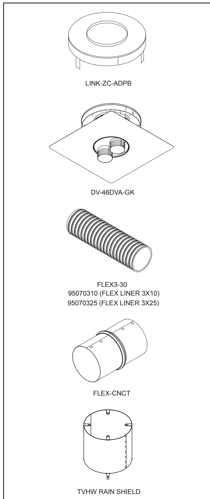
Figure 10.2 Direct Vent Flex Liner Accessory Kits
