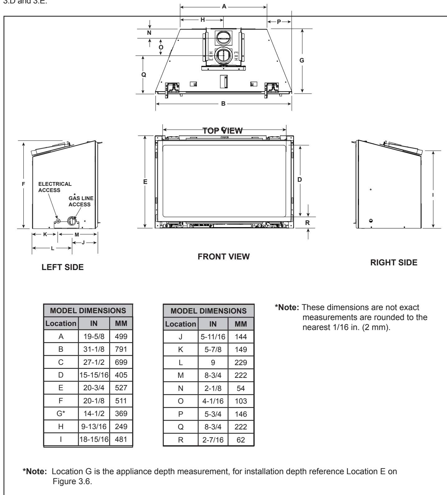
Figure 3.1 Appliance Dimensions
