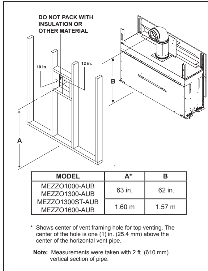
Figure 5.2 Wall Penetration
