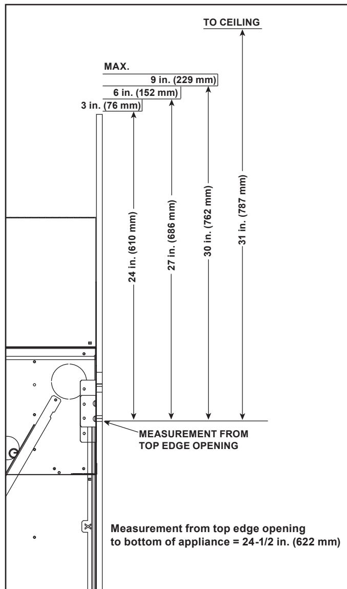
Figure 10.8 Minimum Vertical and Maximum Horizontal Dimensions of Combustibles - MEZZO1600-AUB
