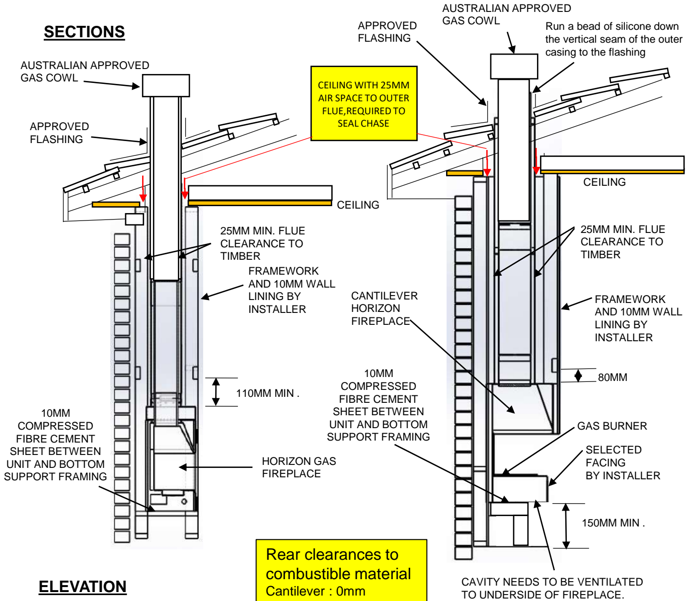
CANTILEVER
